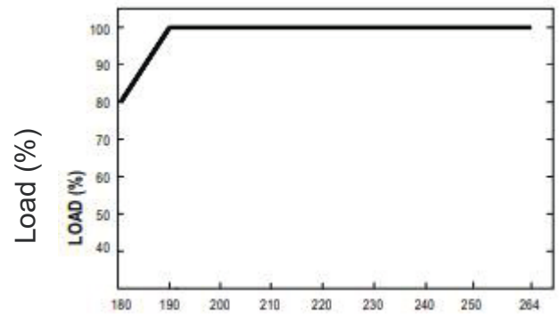
Minus output and input voltage curves
