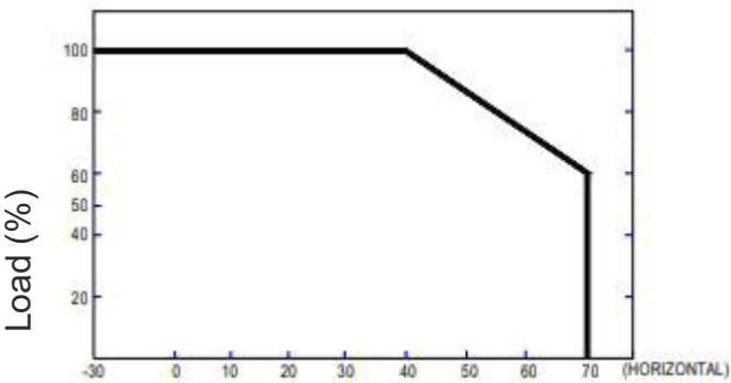
Deducon curve and temperature
