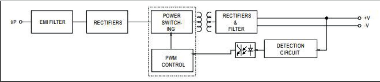
Funconal Diagram
