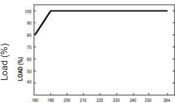
Minus output and input voltage curves
